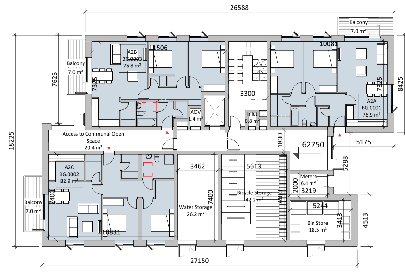
1 Block G Level 00 1:200
