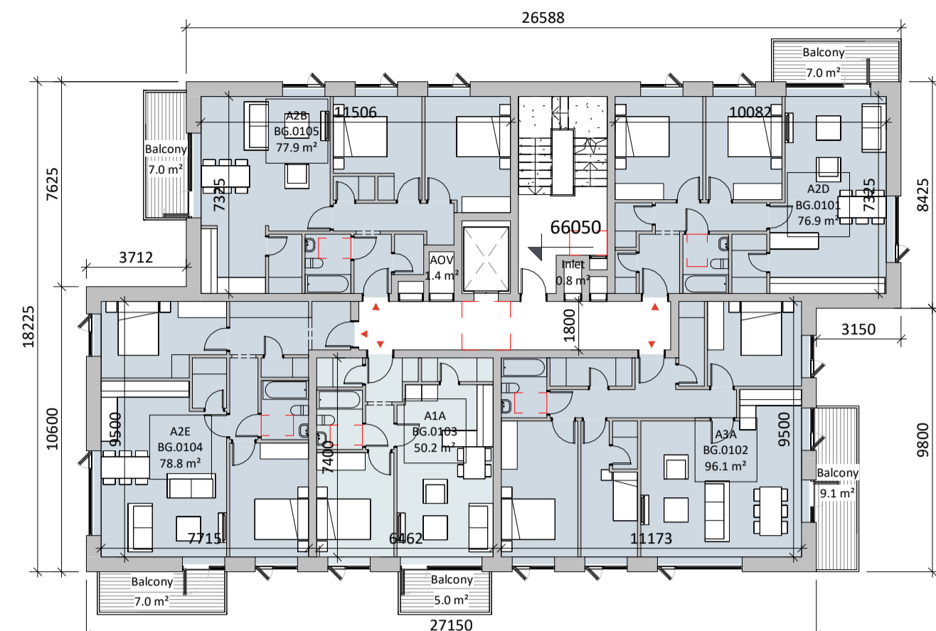
2 Block G Level 01 1:200
