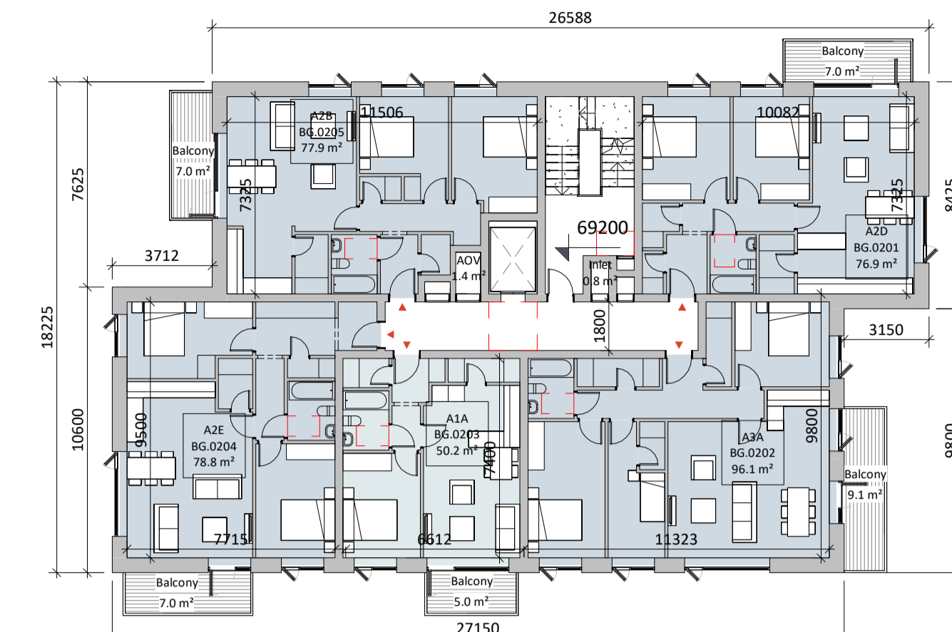
3 Block G Level 02 1:200
