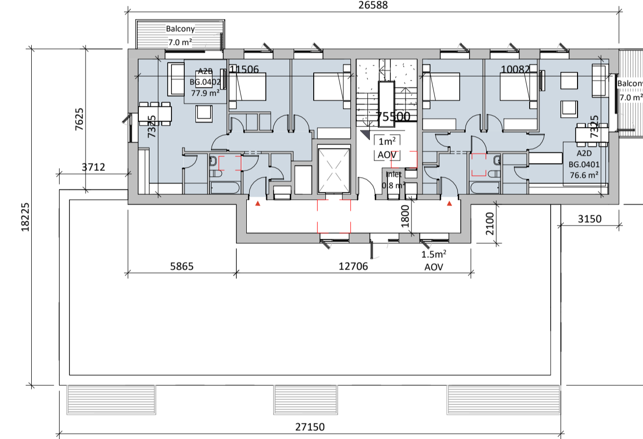
5 Block G Level 04 1:200
